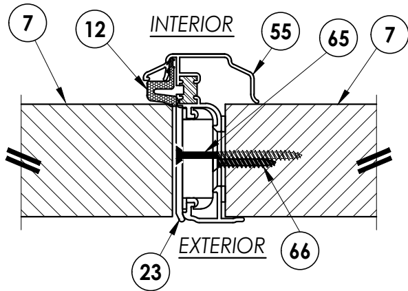
4 HORIZONTAL CROSS SECTION 4 Endura astragal
