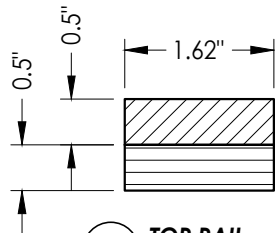
33 TOP RAIL
