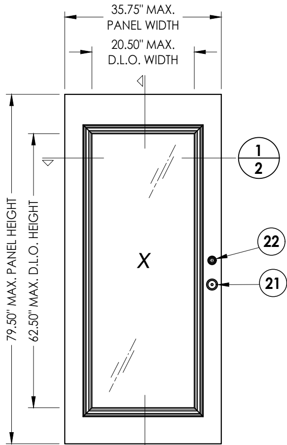
7 FIBERGLASS DOOR Glazed
