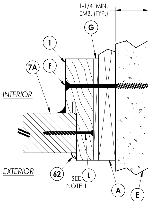
2 HORIZONTAL CROSS SECTION 4 Shown w/1X sub-buck
