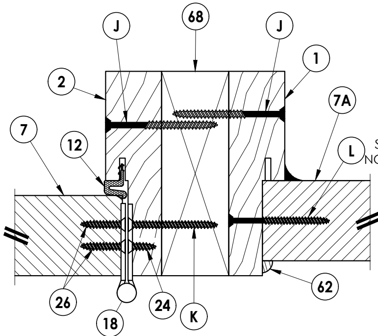
3 HORIZONTAL CROSS SECTION 4
