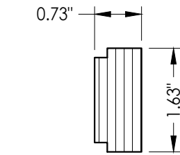
36 LITE OPENING STILE REINF.
