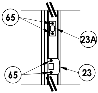
ASTRAGAL DETAIL
